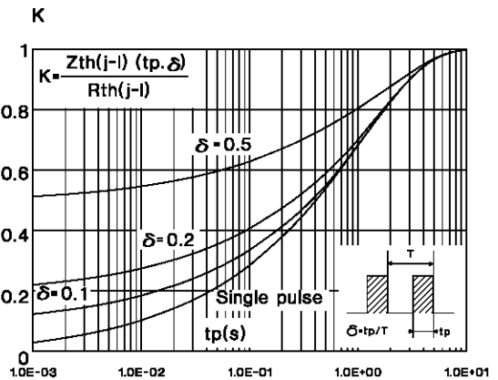
Fig. 14 : Relative variation of thermal transient impedance junction to lead versus pulse duration.
