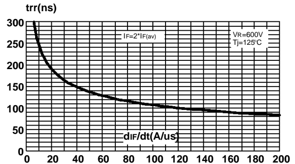
Fig. 16 : Reverse recovery time versus di_F/dt (90% confidence).
